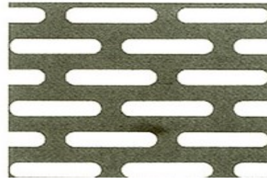
22 4x20 .157"x.787" -41.2% 開孔率
